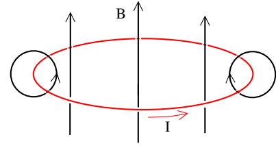
Figure 35: Lenz's law
