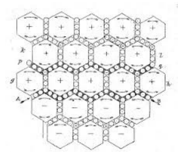
Figure 46: Maxwell's vortices
