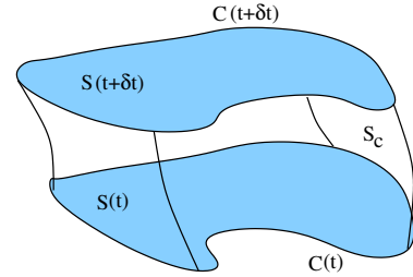
Figure 37: Moving Circuits
